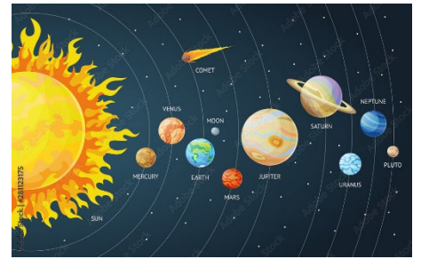
Solar System
