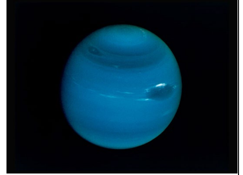
Neptune
