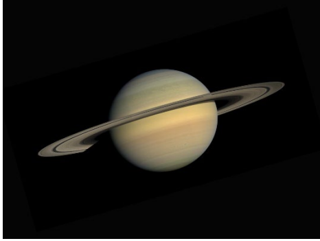
Saturn
