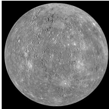
Mercury
