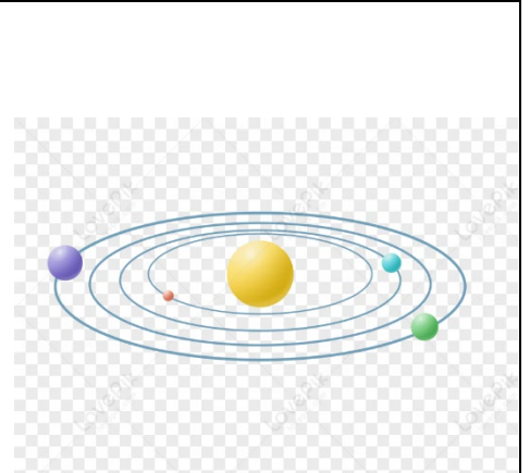
Orbit
