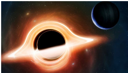
Black hole
