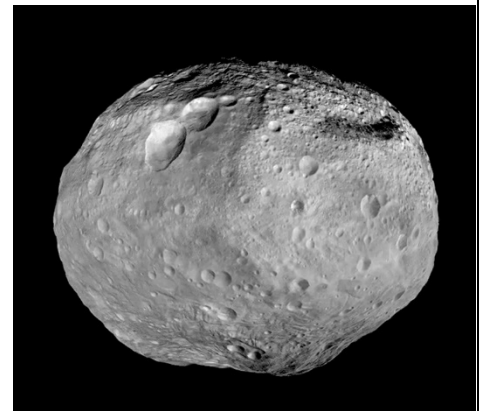
Asteroid
